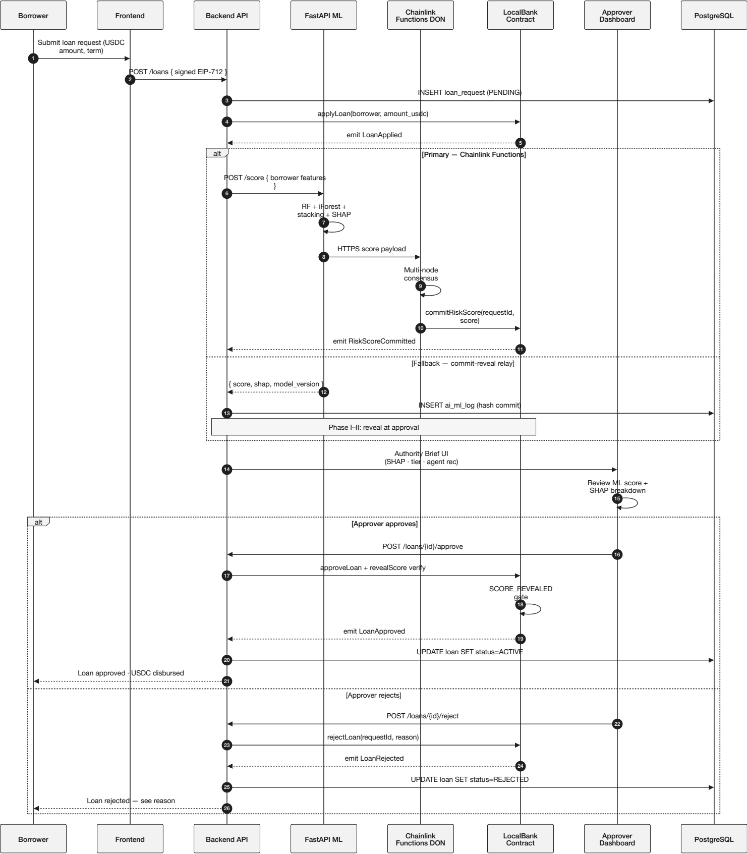
Sequence Diagram — Loan Flow (Functions vs Commit-Reveal · Authority Brief)
